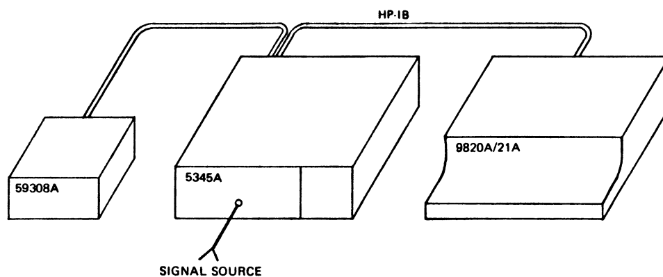
Figure 8. Block Diagram of System to Make a Benchmark
